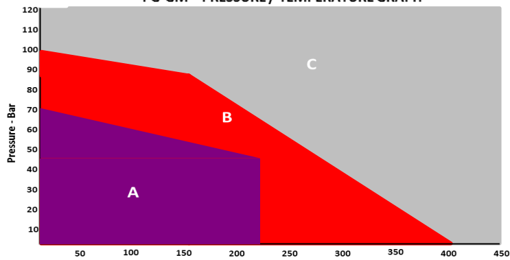
PG-GM – PRESSURE / TEMPERATURE GRAPH
